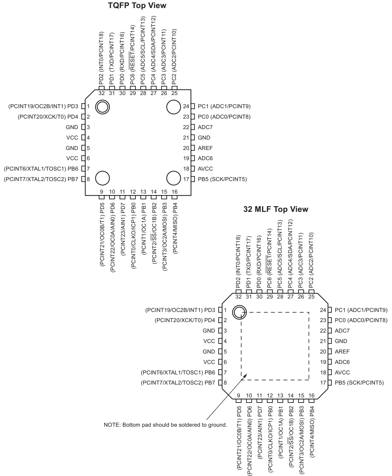
Figure 1-1. Pinout
